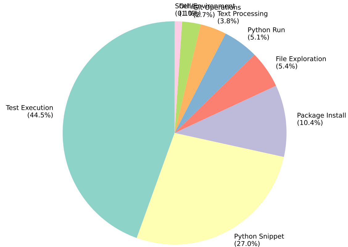
Bash Time by Category
