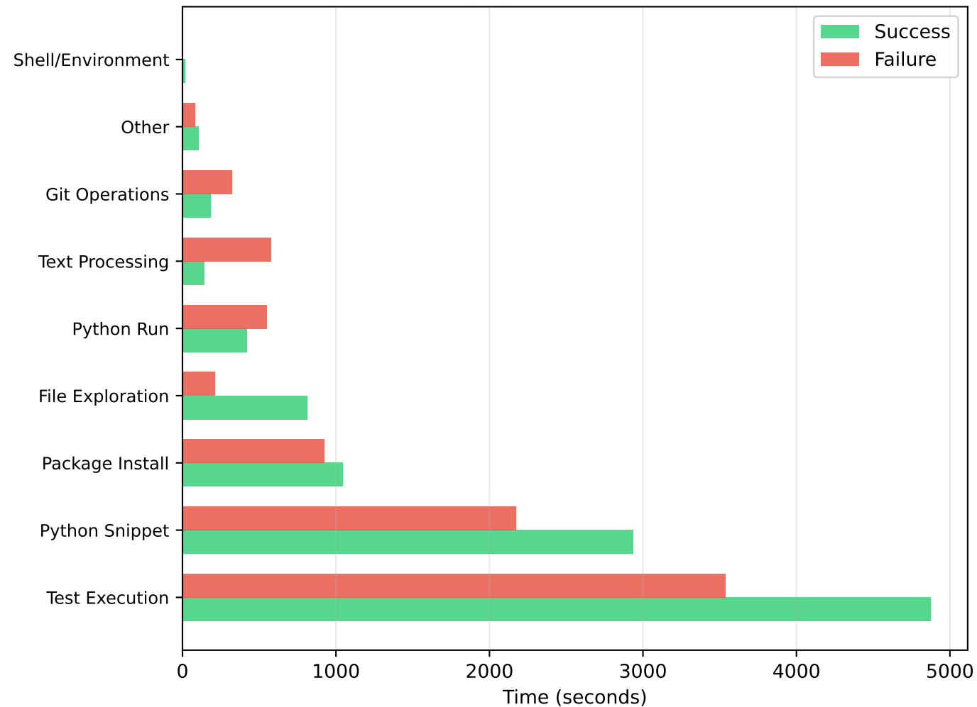
Bash Category Time: Success vs Failure
